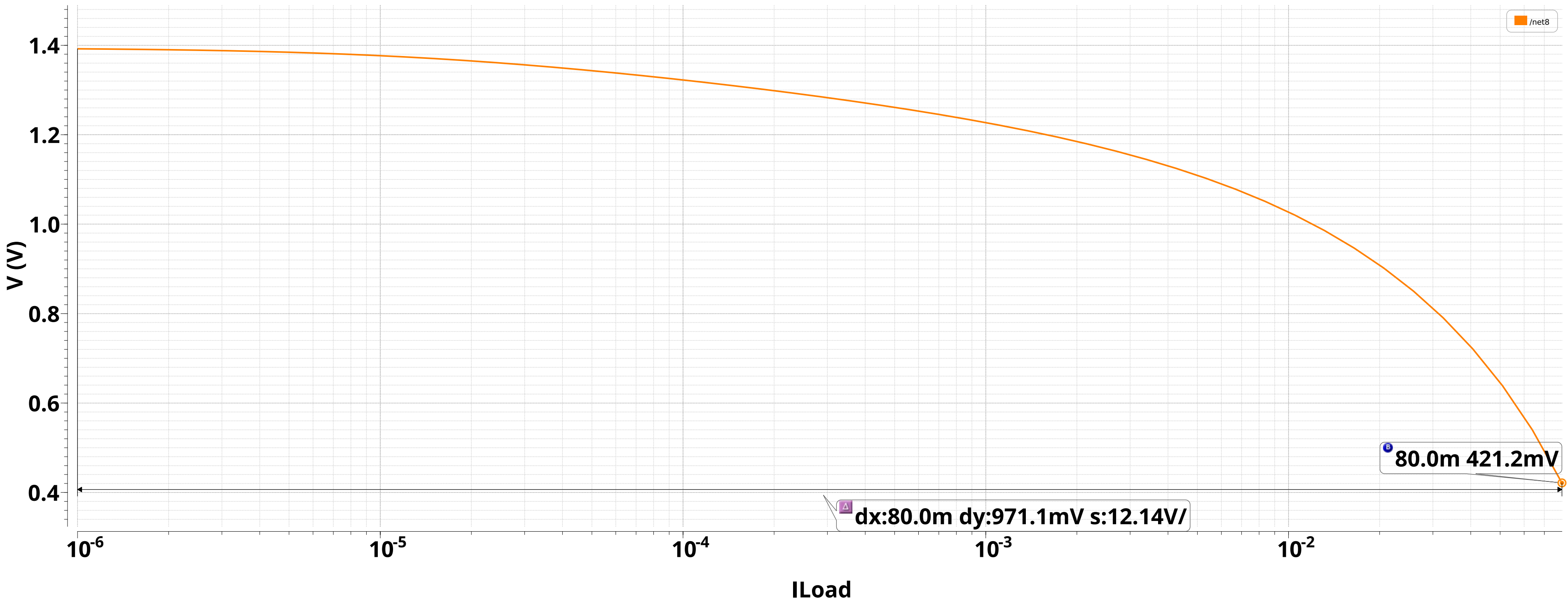
Pass Transistor Gate Voltage vs. Load Current (0->80mA)
